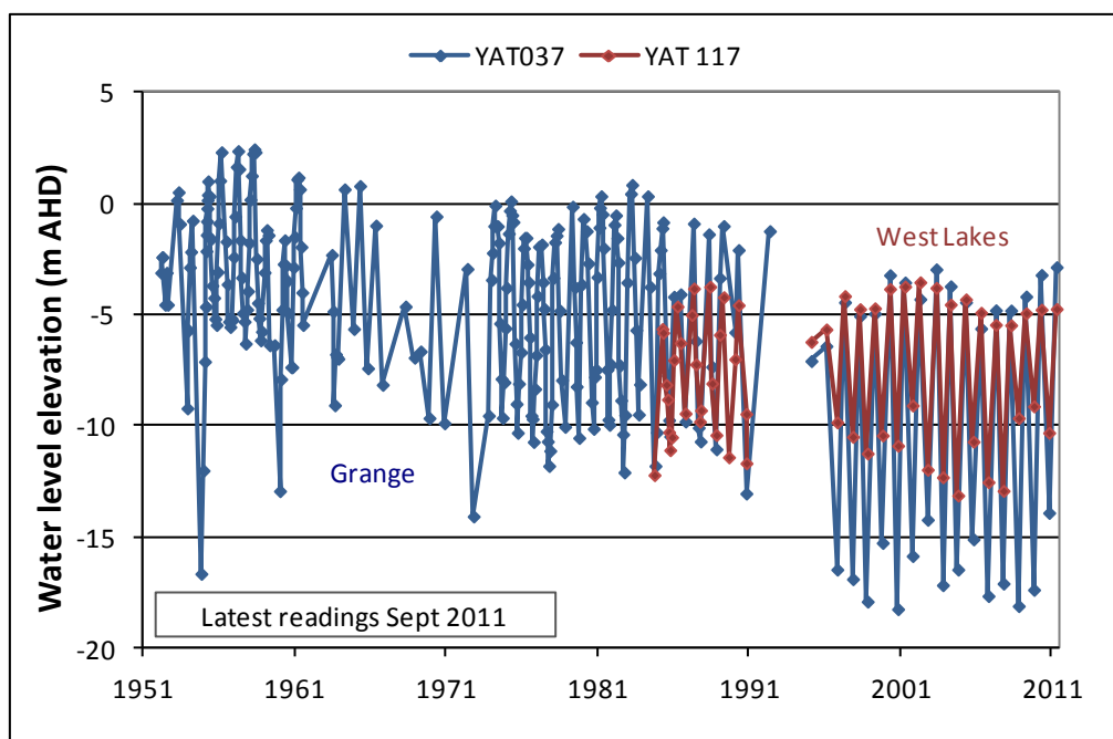
Figure 12. Groundwater level trends for the T1 aquifer in the West Lakes – Grange area of the CAPWA
