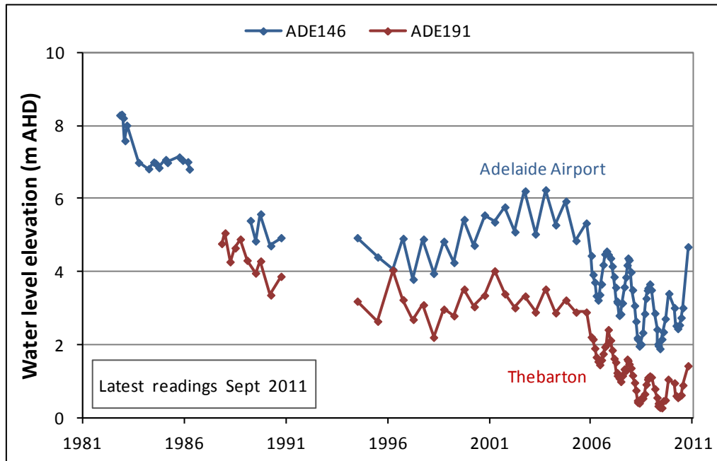
Figure 16. Groundwater level trends for the T2 aquifer in the western suburbs of the CAPWA
