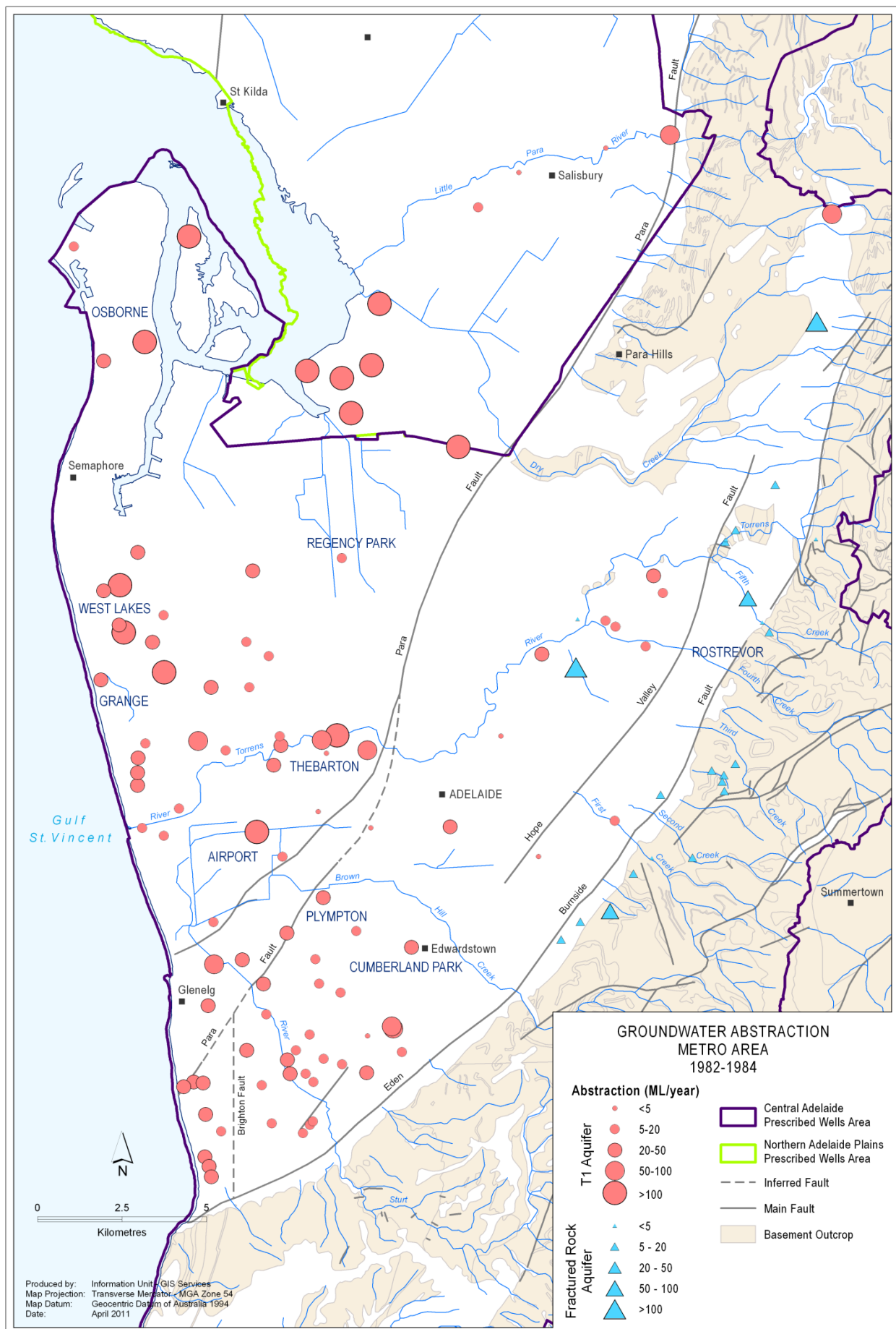
Figure 7. Locations of major groundwater users in the CAPWA
