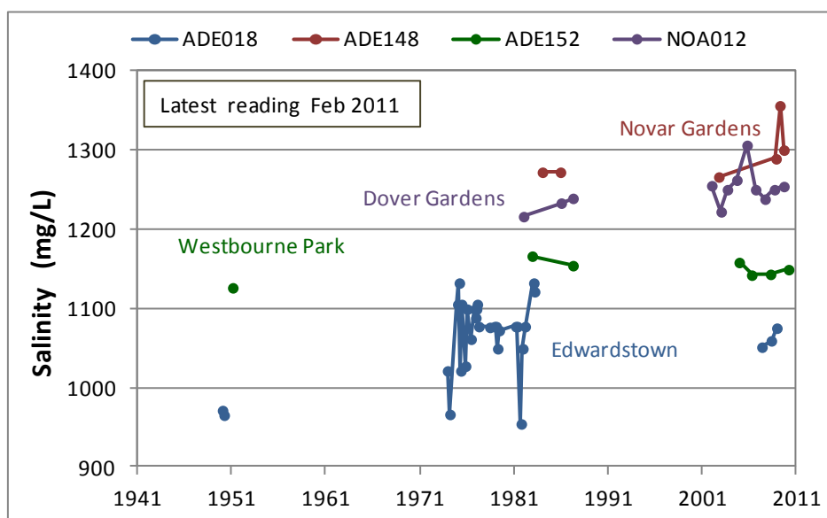
Figure 22. Groundwater salinity trends for the T1 aquifer in the southern suburbs of the CAPWA
