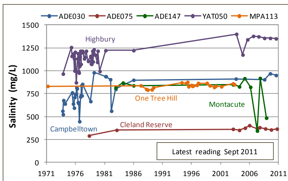
Figure 27. Groundwater salinity trends for the fractured rock aquifer in the CAPWA
