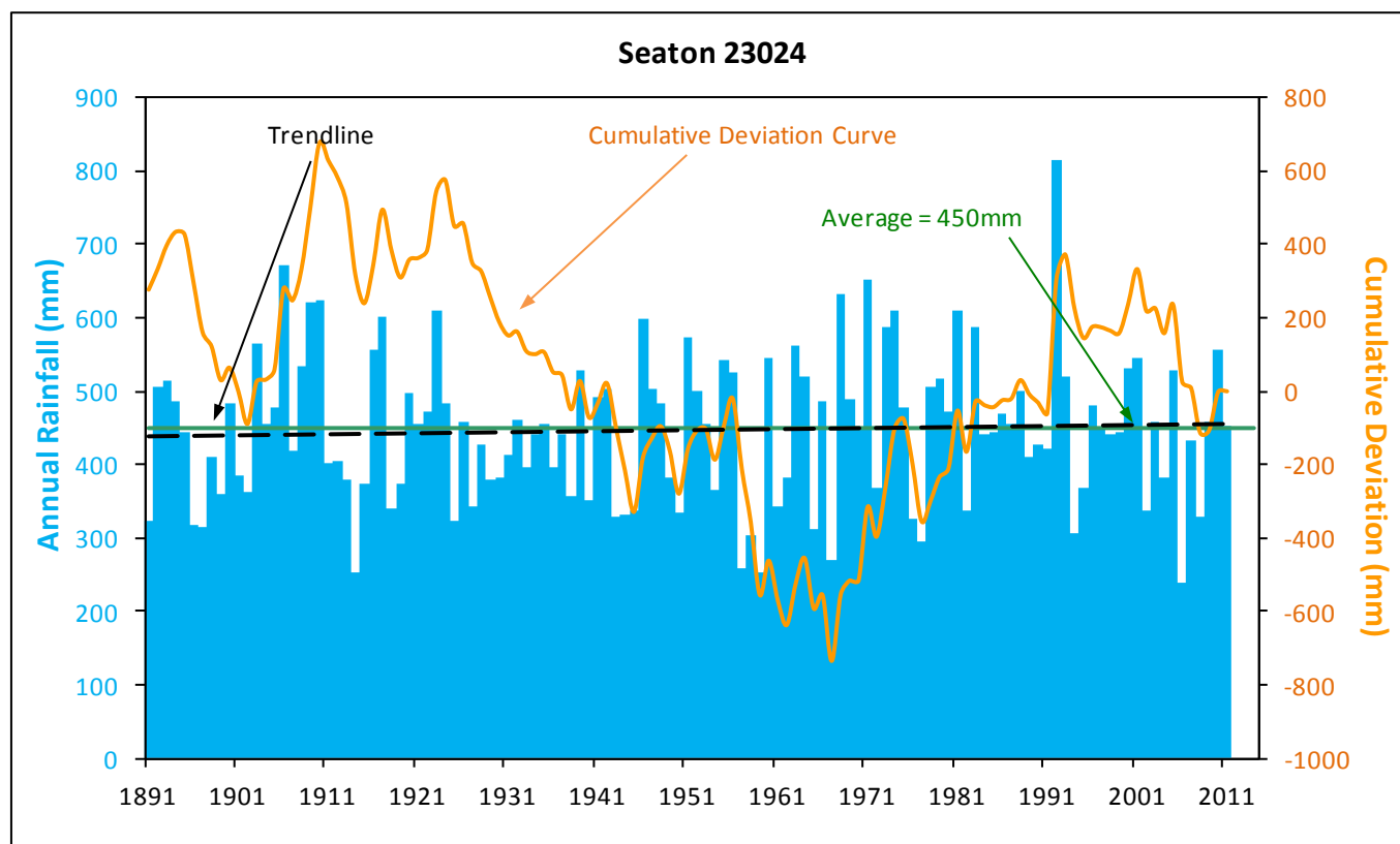
Figure 5. Annual rainfall and cumulative deviation from mean annual rainfall at Seaton in the CAPWA
