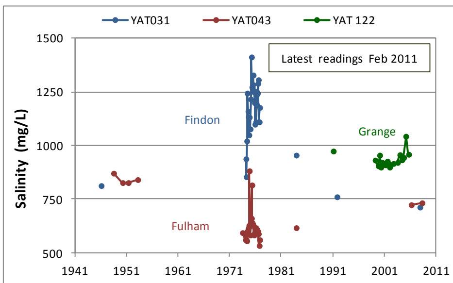
Figure 23. Groundwater salinity trends for the T1 aquifer in the western suburbs of the CAPWA
