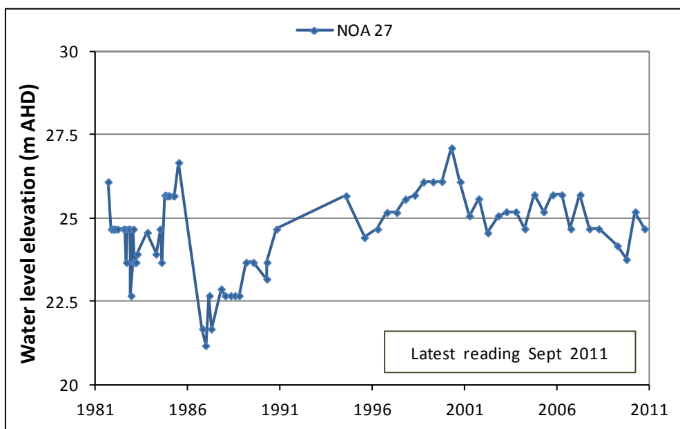
Figure 19. Groundwater level trends for the T4 aquifer in the CAPWA
