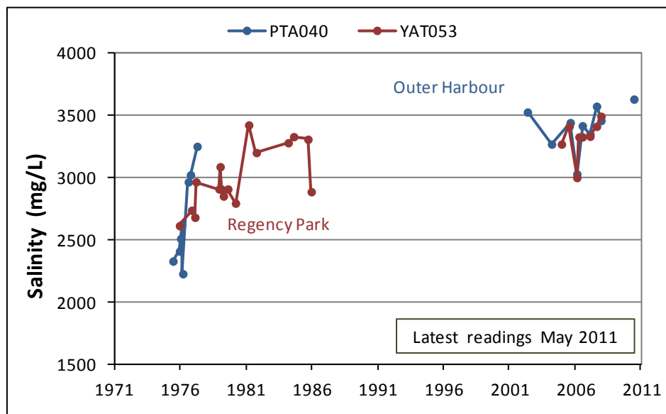
Figure 24. Groundwater salinity trends for the T2 aquifer in the CAPWA
