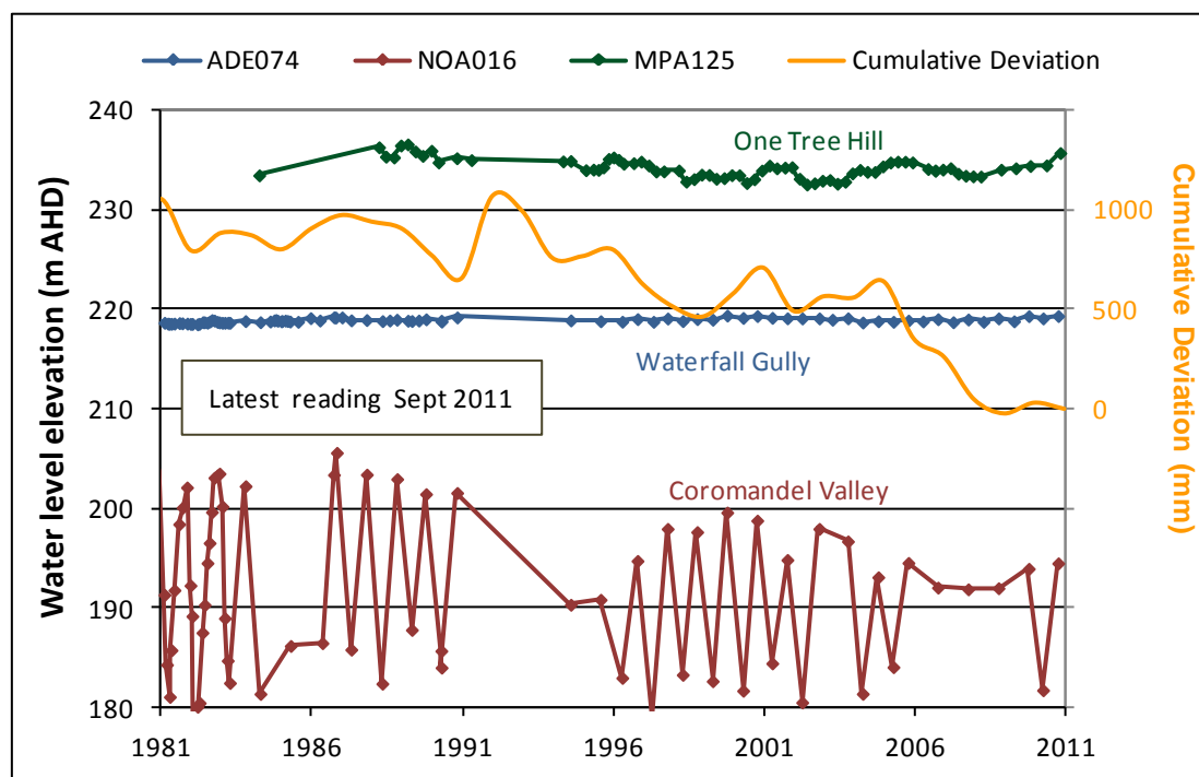
Figure 21. Groundwater level trends for the fractured rock aquifer in the Adelaide Hills region of the CAPWA
