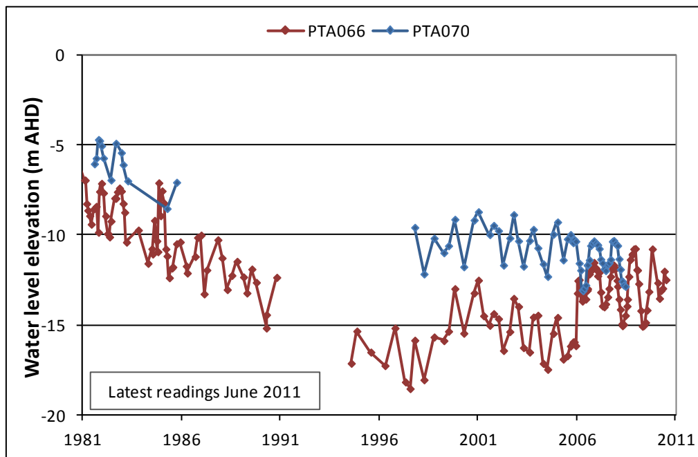
Figure 14. Groundwater level trends for the T1 aquifer in the Osborne area of the CAPWA
