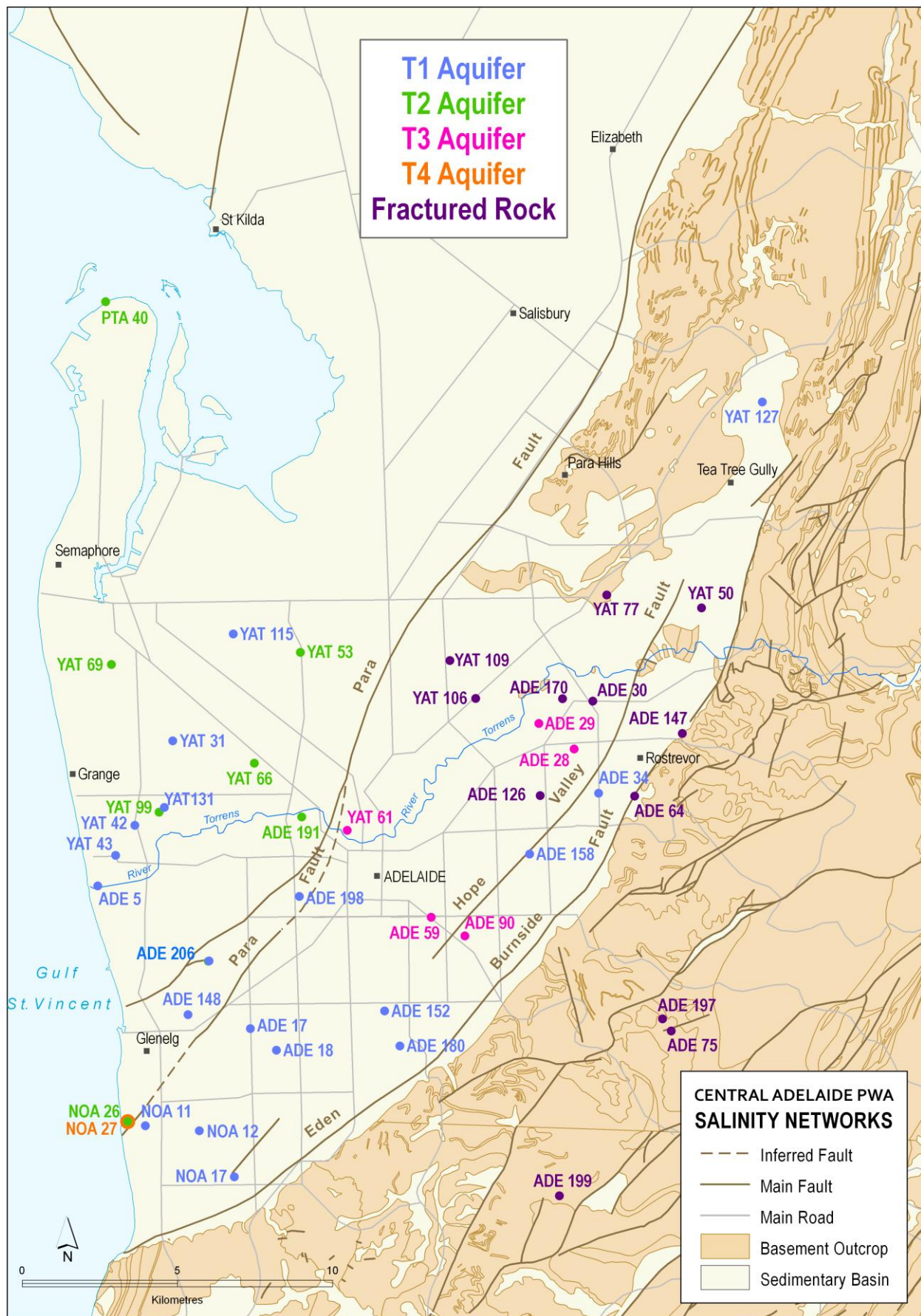
Figure 10. Location of groundwater salinity monitoring wells in the CAPWA
