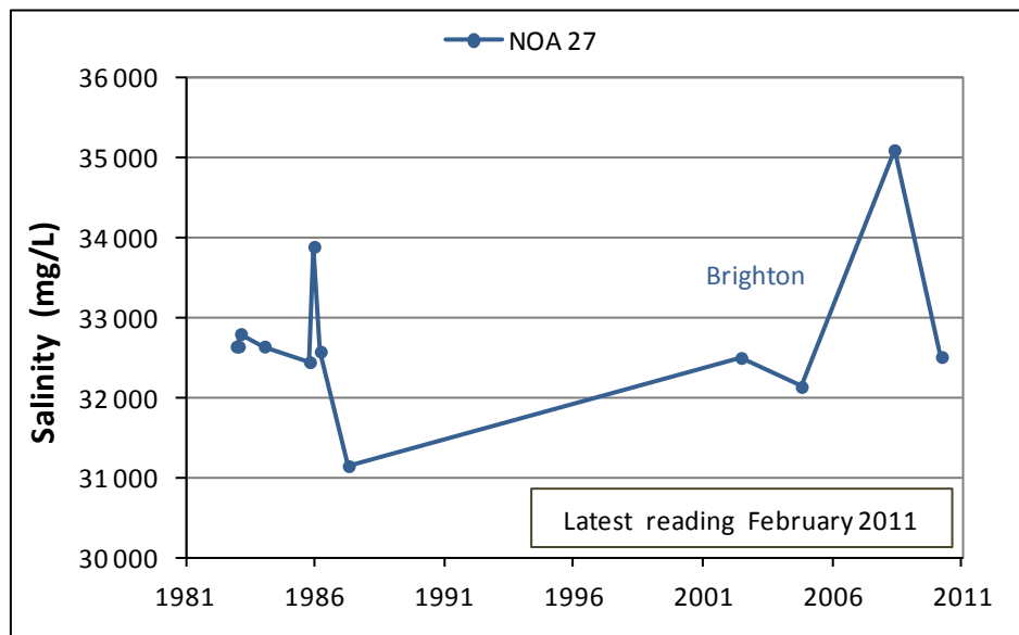
Figure 26. Groundwater salinity trends for the T4 aquifer in the CAPWA
