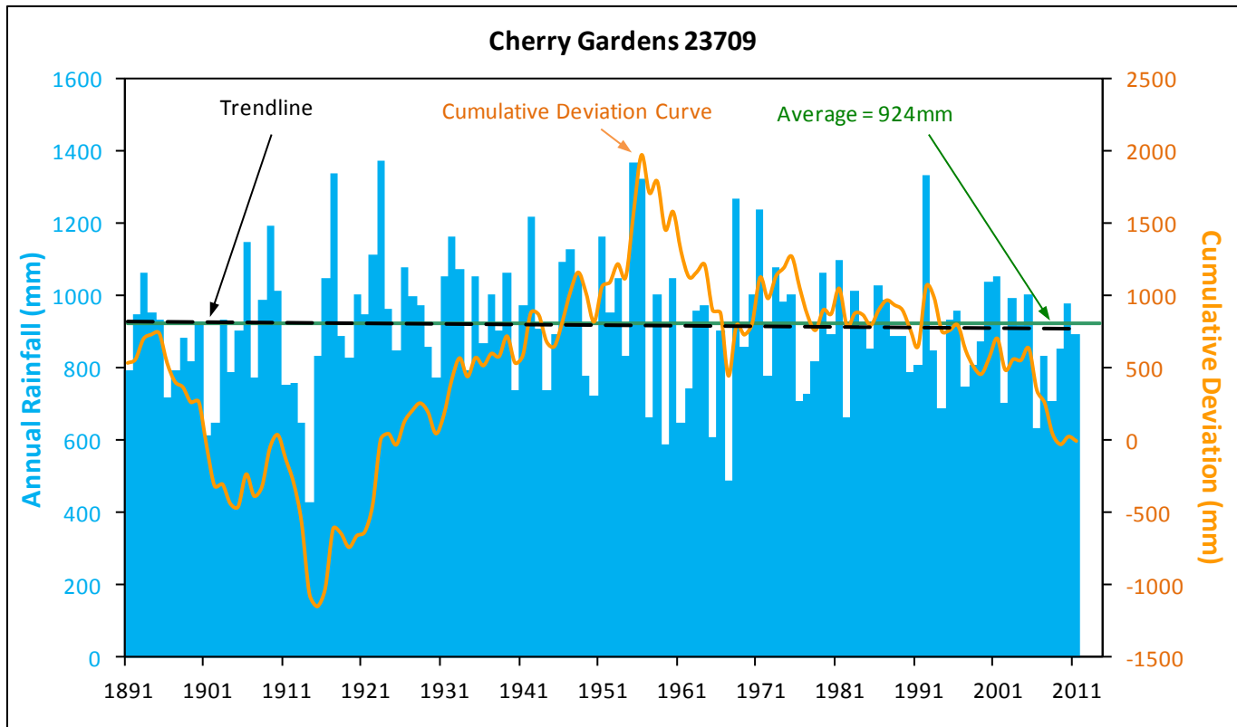
Figure 6. Annual rainfall and cumulative deviation from mean annual rainfall at Cherry Gardens in the CAPWA
