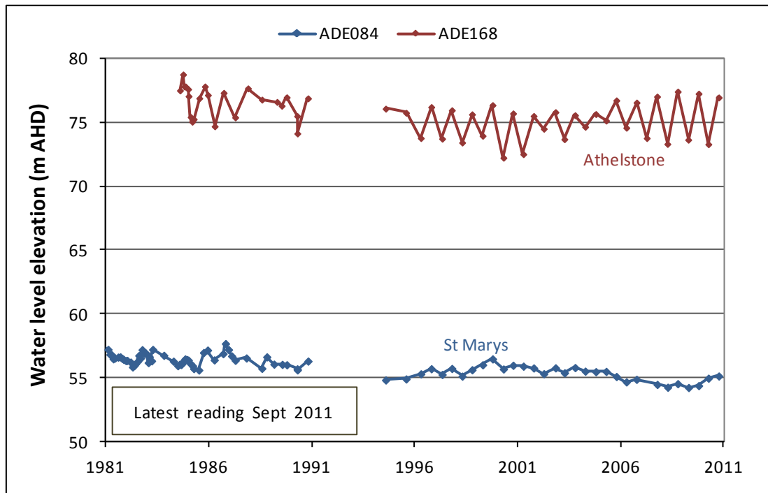
Figure 20. Groundwater level trends for the fractured rock aquifer in the eastern suburbs of the CAPWA
