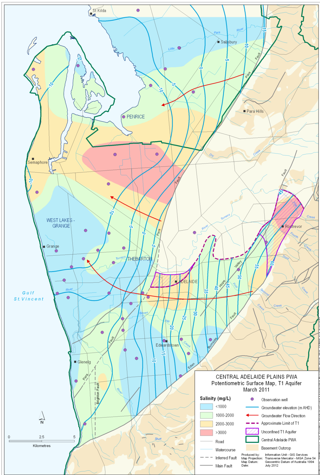
Figure 3. Groundwater-flow direction and salinity distribution (2011) in the T1 aquifer in the Central Adelaide PWA
