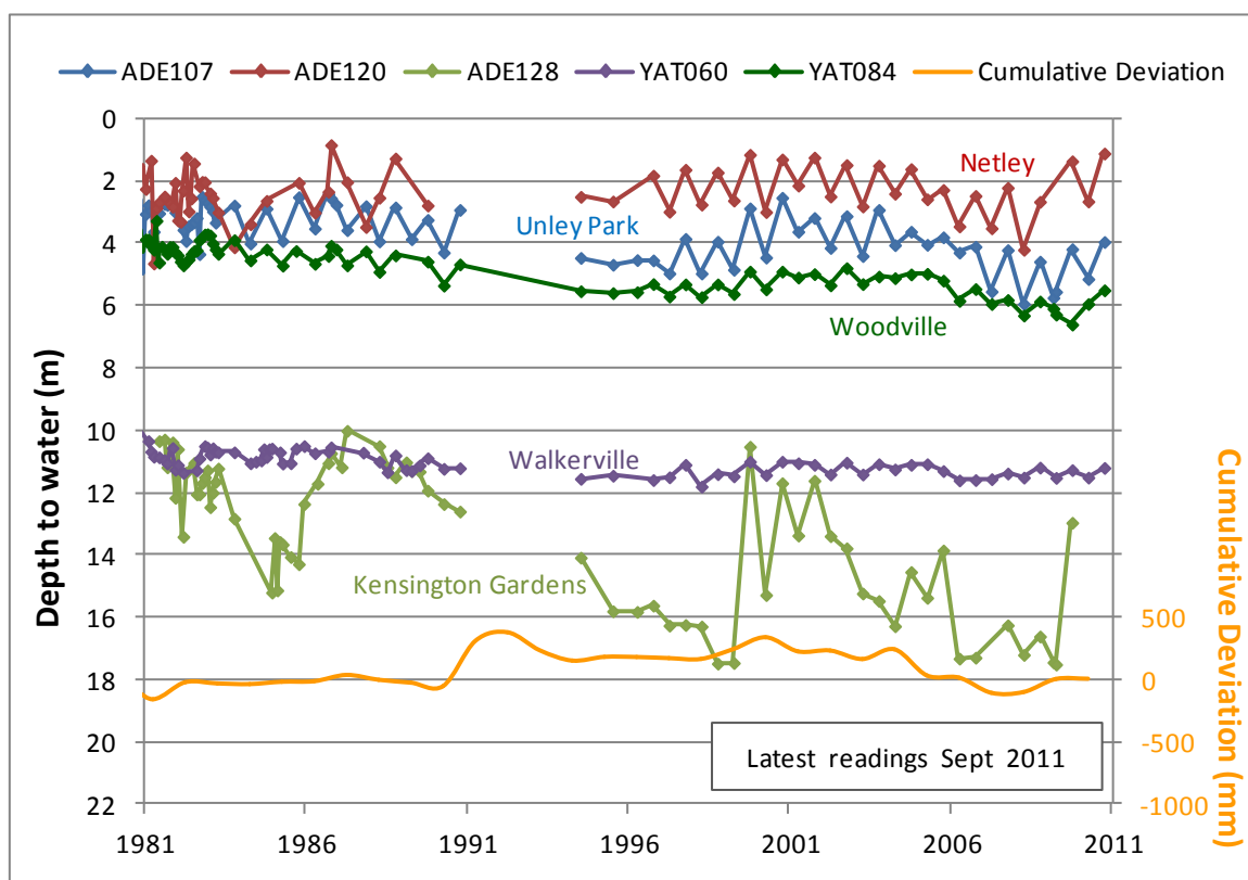
Figure 11. Groundwater level trends for the Quaternary aquifer in the CAPWA
