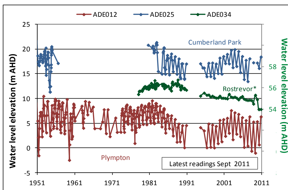
Figure 13. Groundwater level trends for the T1 aquifer in the southwestern and northeastern suburbs of the CAPWA
