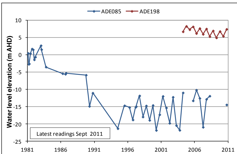
Figure 15. Groundwater level trends for the T1 aquifer in the Thebarton area of the CAPWA
